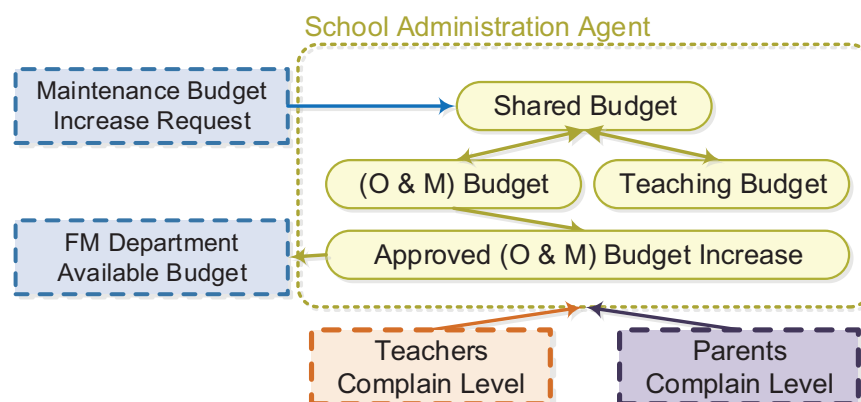
Figure 4.14 School Administration Agent Attributes and Interactions
