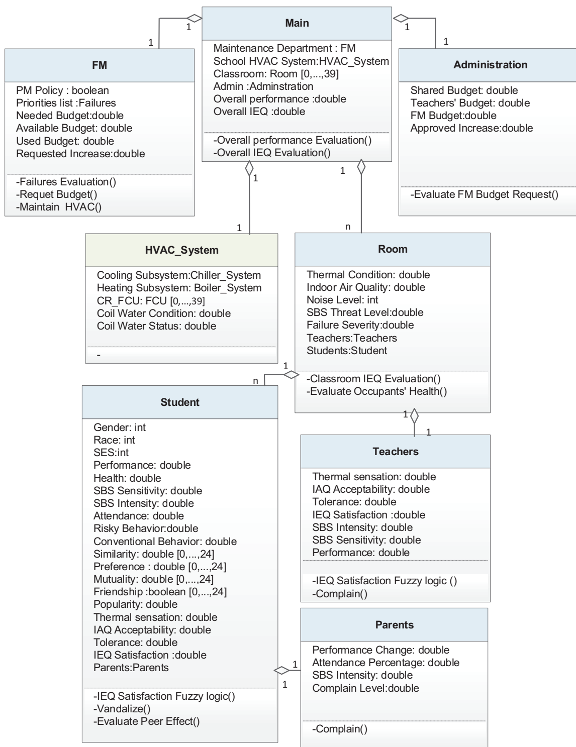
Figure 4.16 General UML Class Diagram
