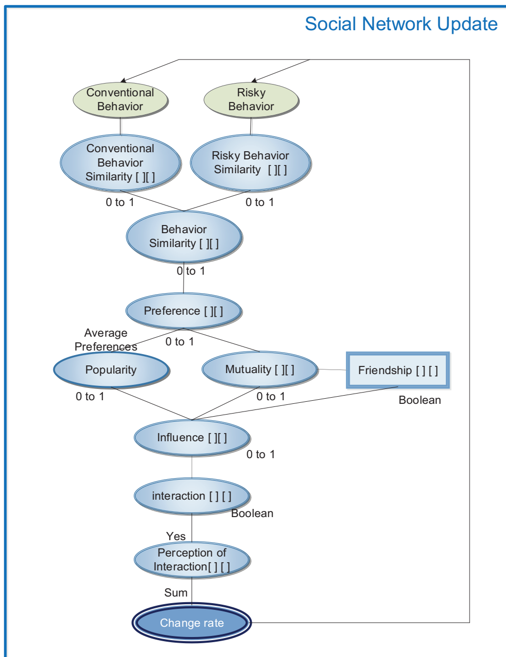
b) Students' Social Network Update Cycle
