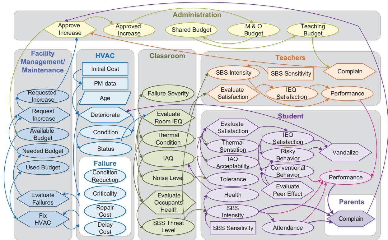
Figure 4.8 Agents' Attributes and Interactions in The Tactical Level Model
